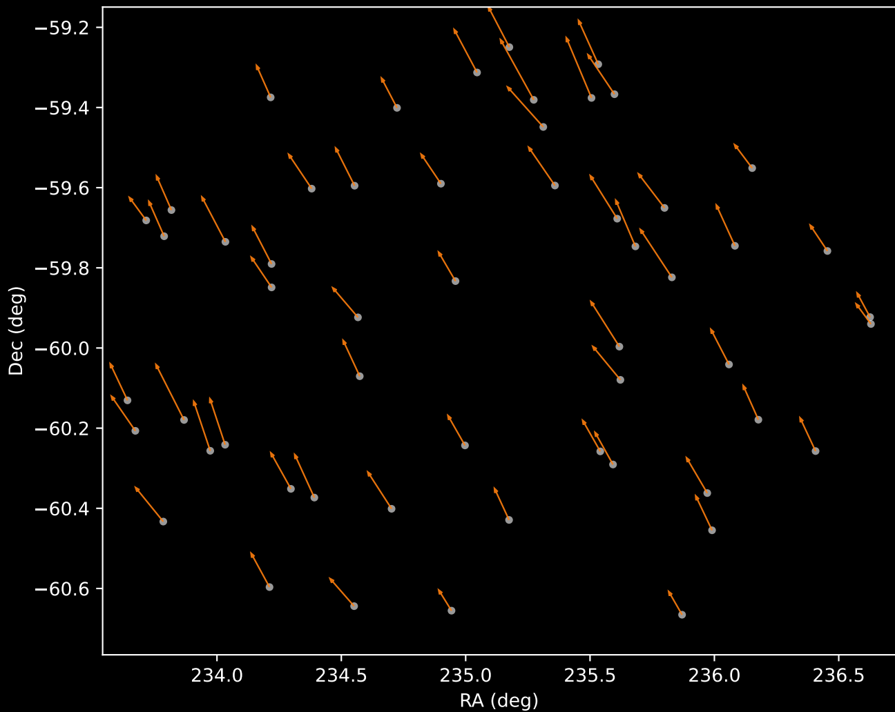
APOGEE DR17 Cluster 2 Proper Motion Vectors (n=55)
