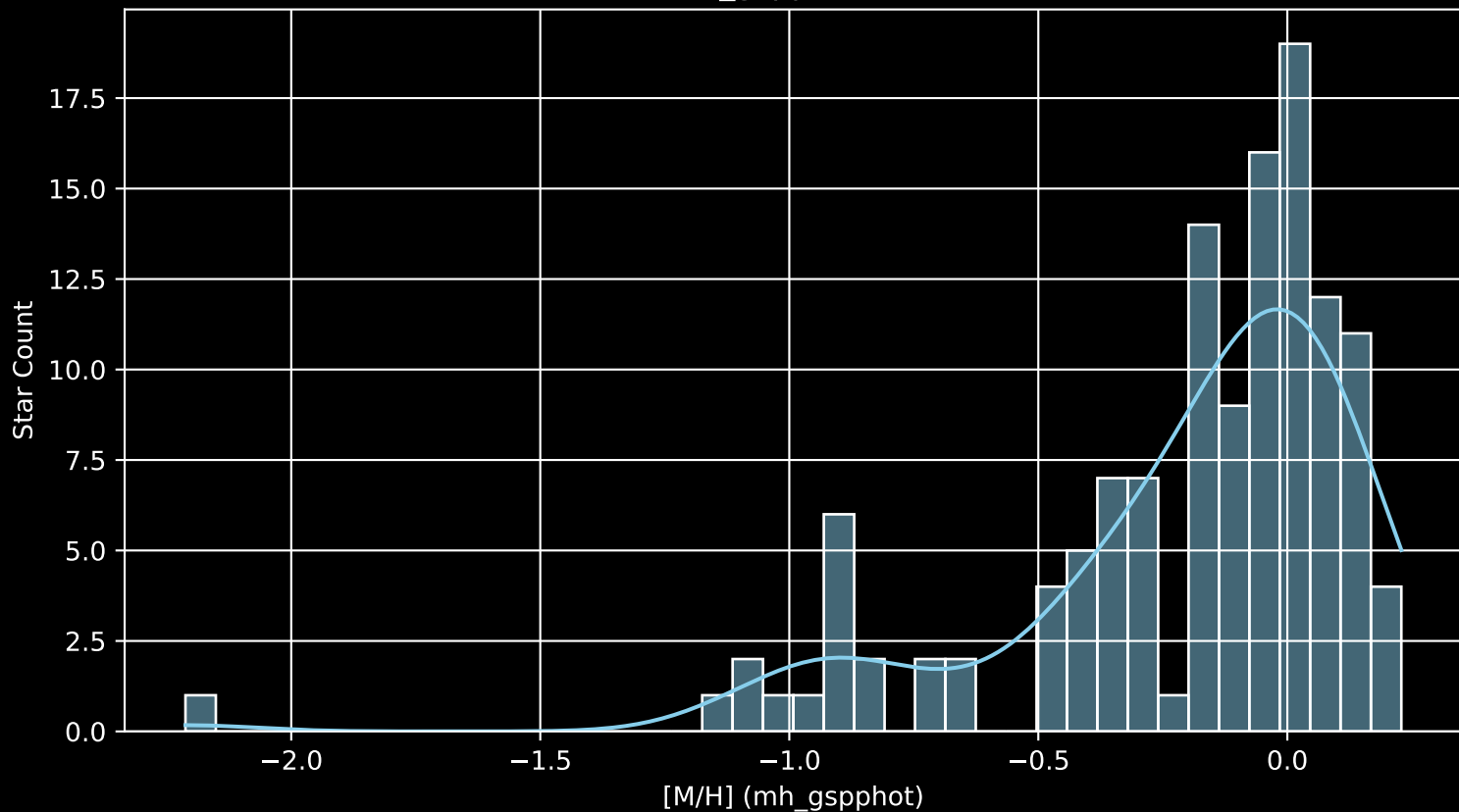
APOGEE DR17 Field: [278-09 [M/H] (mh_gspphot) (n= 127)
