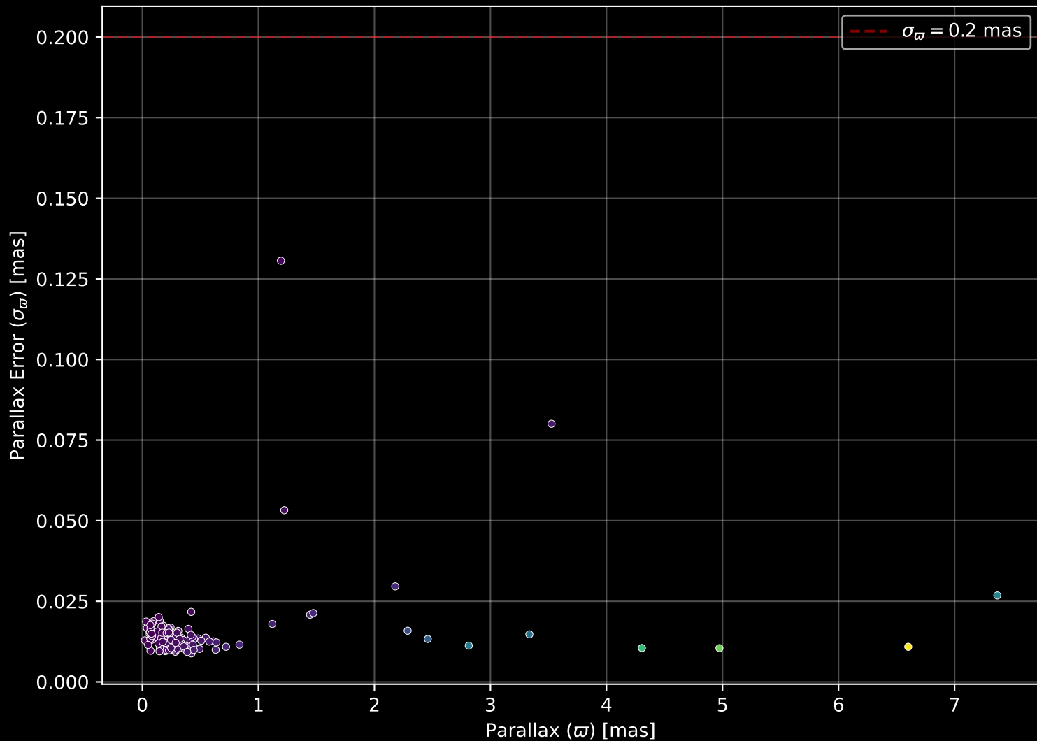
APOGEE DR17 Field: [278-09] Parallax Quality (n= 128)
