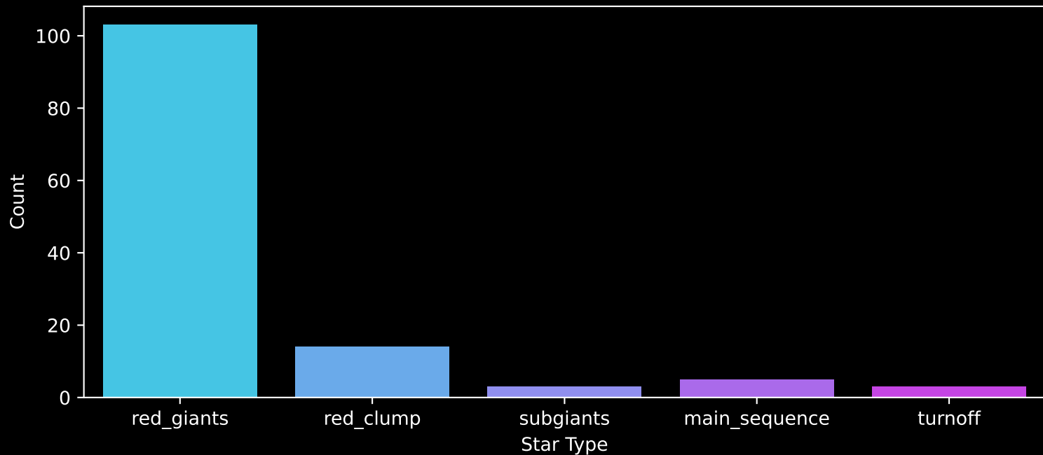
APOGEE DR17 Field: [278-09] Count plot of Star Type
