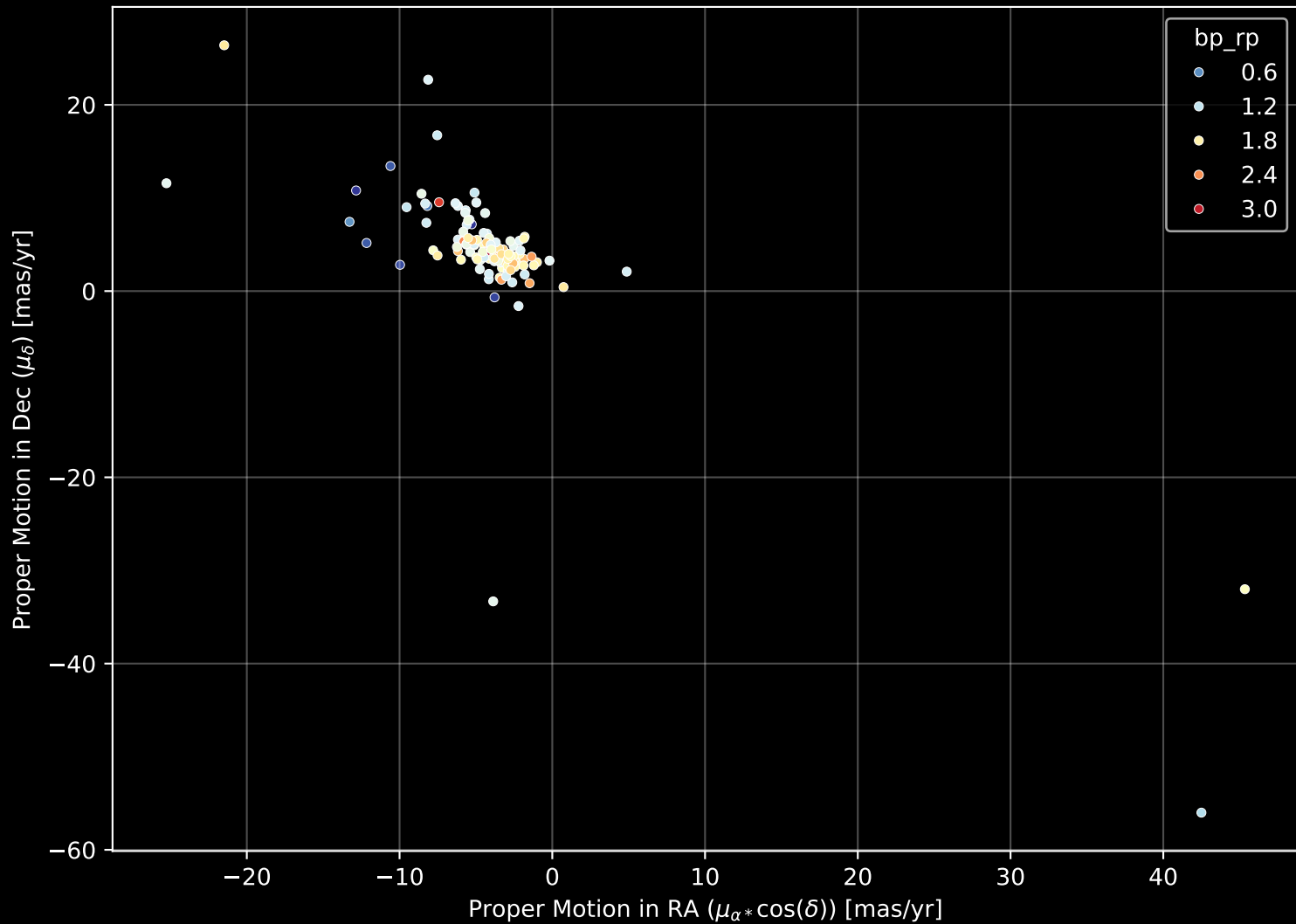
APOGEE DR17 Field: [278-09] Proper Motion Diagram (n= 128)
