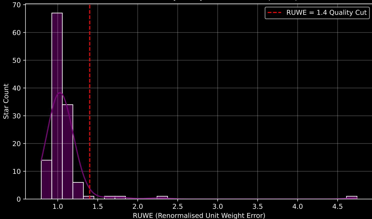
GAPOGEE DR17 Field [278-09] RUWE Distribution (n= 126)
