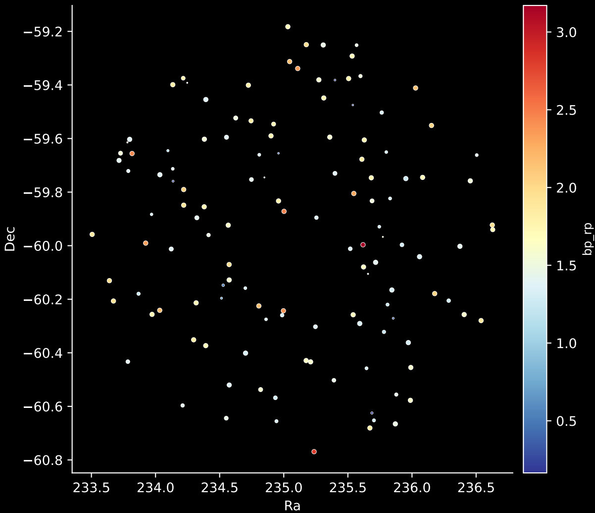
APOGEE DR17 Field: [278-09] Stars: 128
